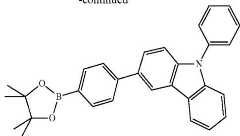
Intermediate 6
