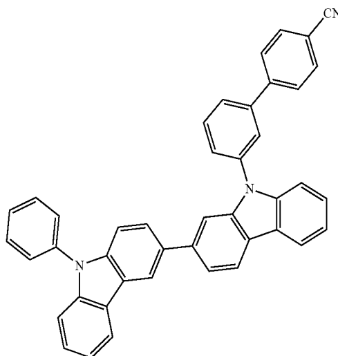
Compound H4
