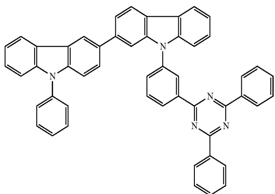
Compound F2
