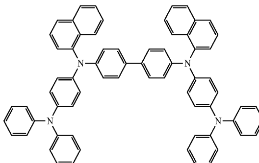
Compound BD2
