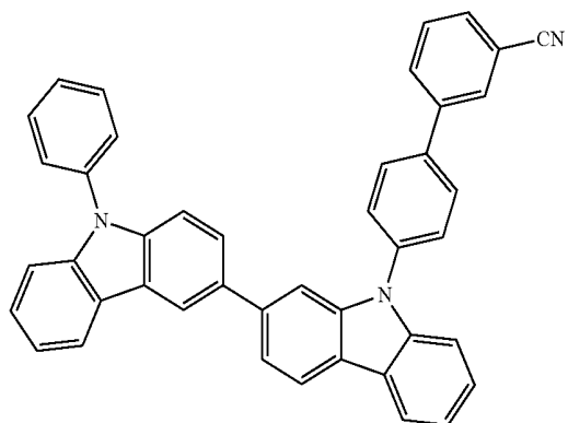
Compound H2
