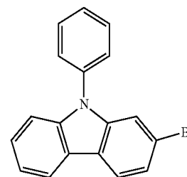
Intermediate 14
