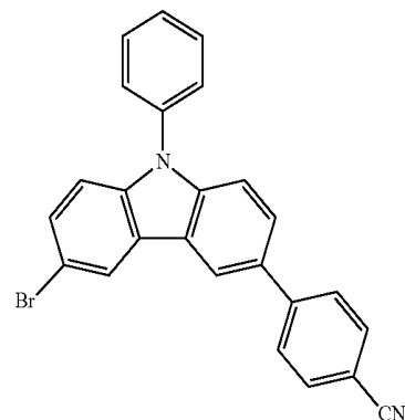
Intermediate 9
