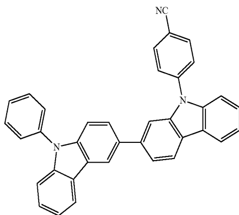
Compound H1
