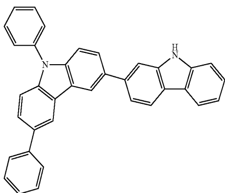
Intermediate 13
