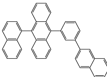
Compound BD1
