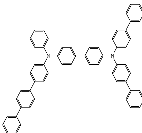
Compound X1
