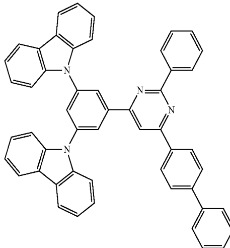
Compound BH1
