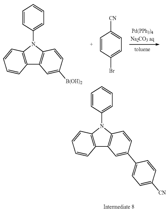
Intermediate 8
