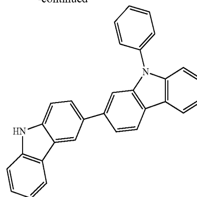
Intermediate 16
