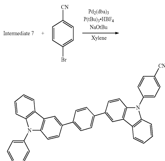
H12
