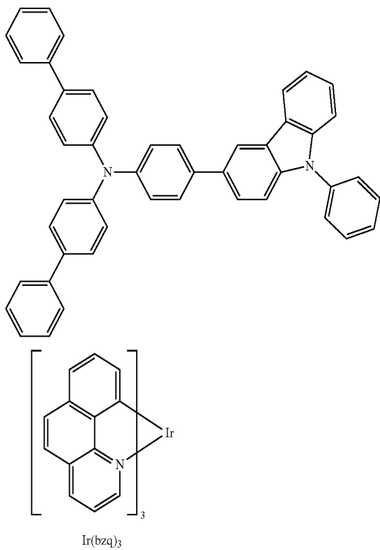
Compound ET
