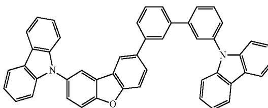
Compound F4
