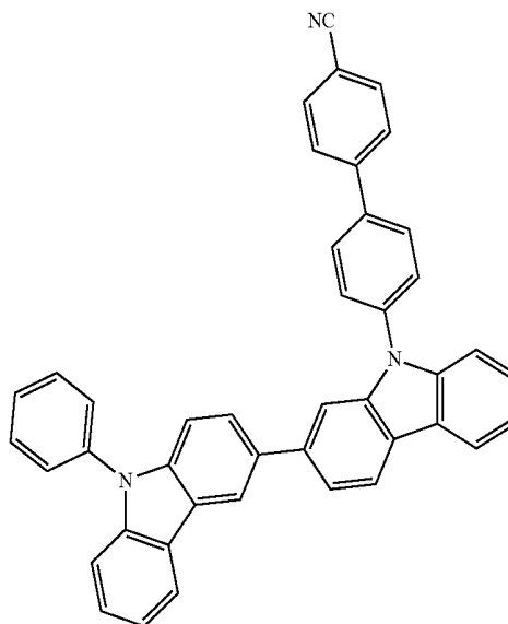
Compound H4
