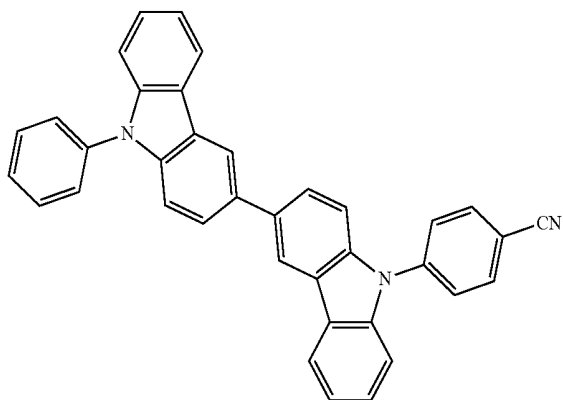
Compound H6
