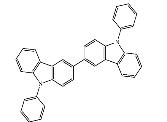
Compound F2
