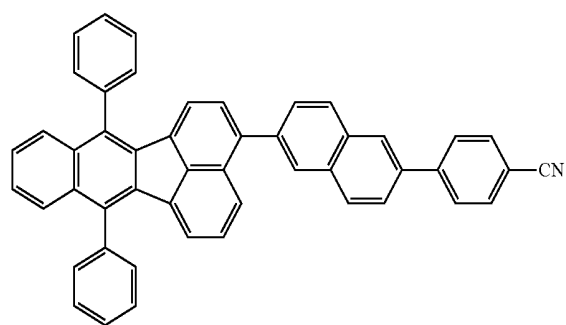
Compound BD1
